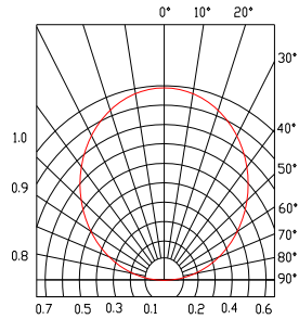
FIG.5 RADIATION DIAGRAM
