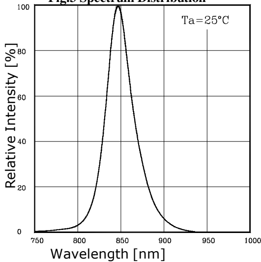
Fig.3 Spectrum Distribution
