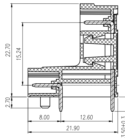
SECTION: P-P
